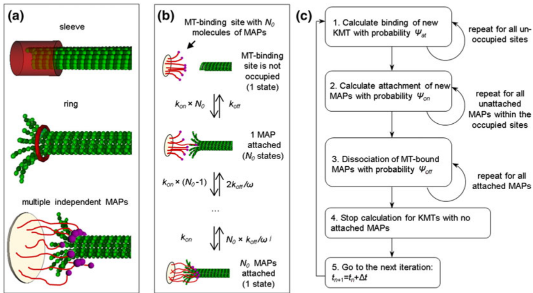
FIGURE 1. Theoretical approaches to study kinetochore–MT interactions. (a) Possible designs of kinetochore–MT binding site. The sleeve and ring models assume that the MAPs are connected rigidly, so their MT binding is not truly independent. In our model, the MAPs can bind and unbind independently, although their apparent dissociation rate is different when two or more MAPs are found next to each other. (b) Schematic of the model for molecular interactions between the MT and N_0 -independent MAPs comprising one MT-binding site. Arrows and their labels correspond to the sums of all possible transitions between two different states, e.g., the MT bound to j and j + 1 MAPs. For details see “ General Model Description ”. (c) Scheme of the stochastic simulation algorithm for model of the entire kinetochore interface with multiple MT-binding sites, see section “ Numerical Simulations of the Kinetochore Interface with Multiple MT-Binding Sites ”.
