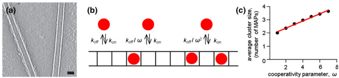
FIGURE 2. Quantitative estimation of the range of cooperativity parameter for NDC80 complexes. (a) Cryo-electron microscopy image of the MTs pre-incubated with soluble NDC80 protein shows the drastically different degree of protein decoration. The length of MT on the left is about 350 nm, which corresponds to 90 NDC80 complexes bound to each protofilament, assuming that NDC80 binds every tubulin monomer. 45 Bar is 25 nm. Reproduced with permission from Alushin et al. 4 (b) Simplified model to estimate the degree of cooperativity that leads to complete decoration of one but not the adjacent MT, as seen in (a). All binding sites are unoccupied at the beginning of simulation; then MAPs (red circles) bind with association rate k_{on} but their dissociation is inhibited due to cooperativity. See “ Model Description ” for details. (c) Plot shows how the cooperativity parameter affects the average size of a cluster of MAPs. Calculated for k_{on} = 1 \text{ s}^{-1} and on average 50% occupancy of the binding sites in the linear array.
