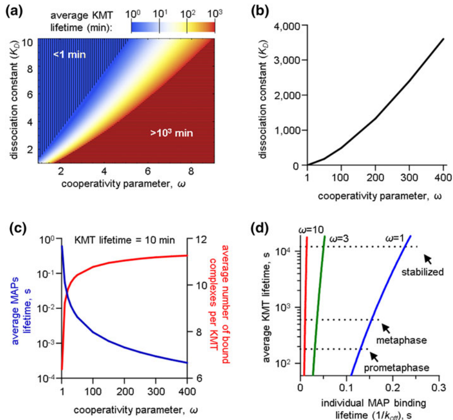
FIGURE 4. Impact of MAP cooperativity on MT-MAP interactions at one MT-binding site. (a) Color chart shows the dependency of average lifetime of MT attachment at MT binding site on the values of cooperativity parameter \omega and dissociation constant K_D . See legend to Fig. 3a for details. (b) Plot shows values of the cooperativity parameter and dissociation constant K_D that produce average KMT lifetime 10 min, mimicking the KMTs in metaphase PtK1 cells. (c) Blue curve shows how the average lifetime of MAP’s binding depends on the cooperativity parameter at the physiological rate of KMT turn-over (10 min). Red curve shows the average number of MT-bound MAPs per KMT for different values of cooperativity. (d) Dependence of the average KMT lifetime on the lifetime of individual MAPs was calculated for k_{on} = 10 \text{ s}^{-1} . For \omega > 10 the data are not shown because the curve practically merges with the Y axis.
