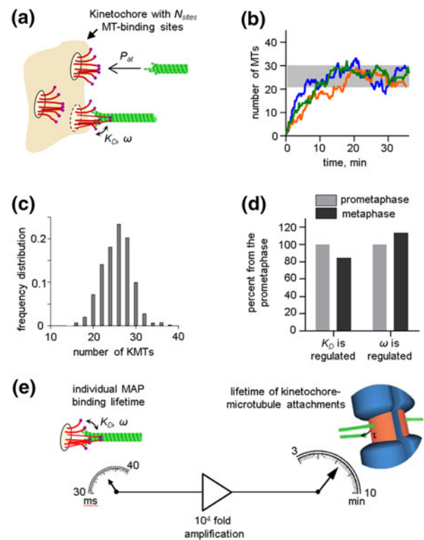
FIGURE 5. Model of kinetochores interface with multiple MT-binding sites. (a) Schematic of the kinetochores interface with multiple MT-binding sites (only part of the kinetochores is shown). After MT encounters one of the binding sites with probability P_{\text{at}} , it immediately initiates molecular interactions with all MAPs within this site. Values of model parameters that were used to obtain results in this figure are listed in Table 1. (b) Results of three independent simulations of the kinetochores model. Time zero is a start of calculation, corresponding to the initiation of MT binding to the kinetochores. Grey bar indicates the range for the number of KMTs that was found at metaphase in PtK1 cells. 26 (c) Distribution of the number of MTs per kinetochores in the model with multiple MT binding sites at steady-state. The average predicted KMT number is 25.6 per kinetochores, consistent with structural studies in PtK1 cells. 26 (d) This graph illustrates how molecular parameters K_D or \omega need to be adjusted to provide the observed stabilization of KMT attachments during metaphase. The average KMT lifetimes in prometaphase and metaphase were 3.5 and 10 min, respectively. 11,13 The average KMT lifetime in prometaphase was obtained for K_D = 3.2 and \omega = 3 ; to calculate average KMT lifetime in metaphase, for columns “ K_D is regulated” the value of \omega was not changed, and K_D was found to be 2.7, which is 84% of the prometaphase value. For “ \omega is regulated” columns the value of K_D was not changed, and \omega was found to be 3.4, which is 113% of its prometaphase value. (e) Schematic that illustrates quantitative relationship between two time-scales in the model: the lifetime of molecular interactions (microscopic parameters K_D and \omega ) and average KMT lifetime (experimentally measured KMT turnover rate).
