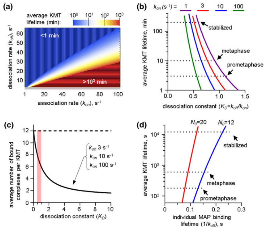
FIGURE 3. Analysis of a model with single MT-binding site in case of non-cooperative binding. (a) Two-colored chart shows average KMT lifetime at one site with MAPs that bind the MT with indicated association and dissociation rates. Horizontal hatching corresponds to highly unstable MTs with lifetimes <1 min. Vertical hatching corresponds to overly stabilized MTs with lifetimes > 10^3 min. Gray bar at the bottom of the plot indicates the region with model solutions for k_{off} < 2 s^{-1} , which was excluded from subsequent analysis. (b) Plots show the relationship between average KMT lifetime and dissociation constant K_D for individual MAPs in a MT-binding site for indicated values of k_{on} . Curve for k_{on} = 1 s^{-1} corresponds to model solutions for which k_{off} < 2 s^{-1} , so they were excluded from further analysis. One can see that the impact of absolute value of k_{on} on this dependence is small. “Stabilized” MTs have lifetime 200 min; such stable KMTs are not seen during normal mitosis but can be obtained when Aurora B kinase, which is one of the major MT-destabilizing factors, is inhibited. 11 (c) Plots show how the number of NDC80 complexes per KMT depends on the value of dissociation constant for three different values of k_{on} . The predicted results do not depend on the value of k_{on} , so the curves overlap completely. Broken line shows the maximum number of NDC80 complexes per site. Pink bar shows the range of K_D that corresponds to the physiological KMT stability. (d) Dependence of the average KMT lifetime on the lifetime of individual MAPs was calculated for K_D values from 0.4 to 1; these values correspond to 6–8 MAPs bound to one MT at steady-state (pink vertical bar in (c)). This plot was obtained for k_{on} = 10 s^{-1} but similar results were obtained for k_{on} ranging from 1 to 100 s^{-1} . Different colors show model solutions for different number of MAPs per MT-binding site (12 and 20).
